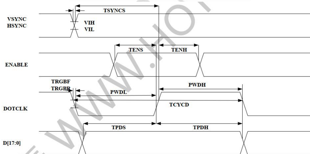
RGB Interface Characteristics
