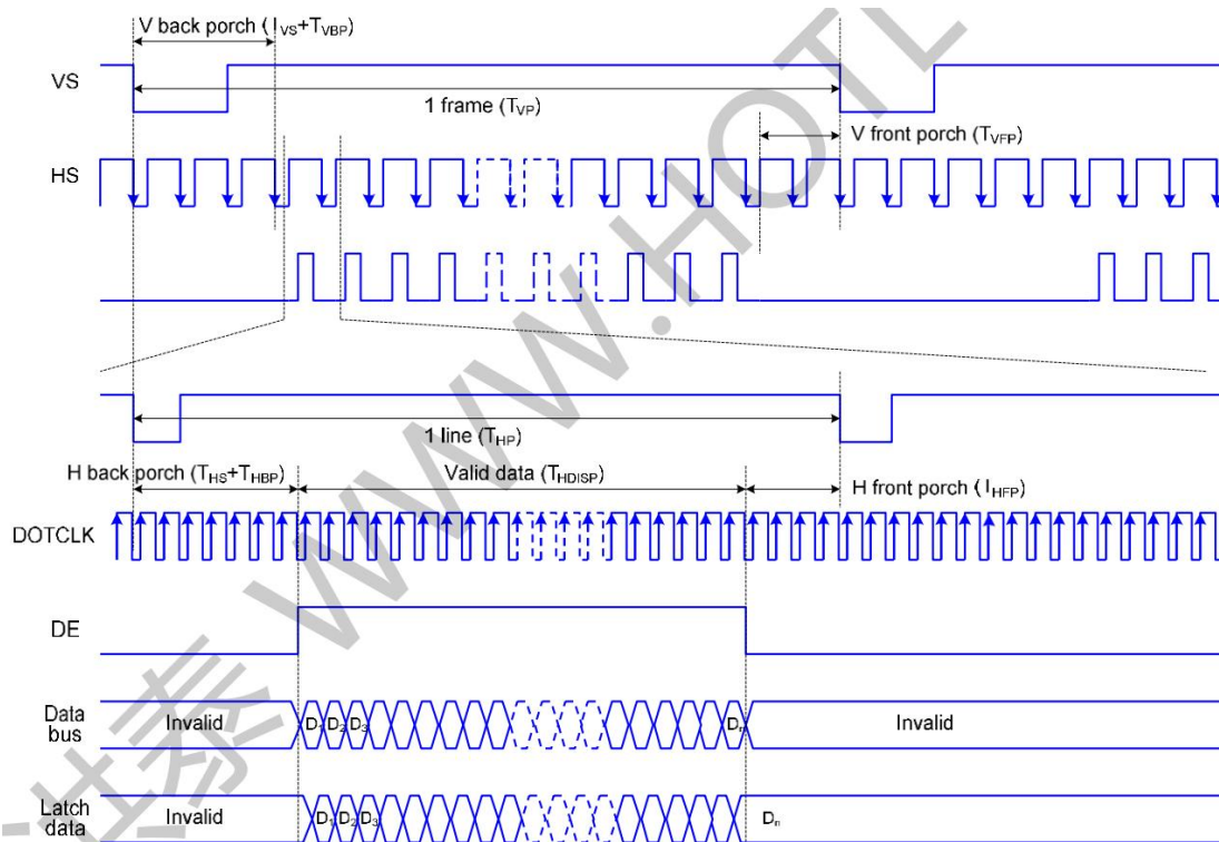
RGB timing diagram
